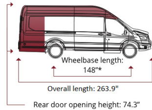
Transit 148 Ext HR
